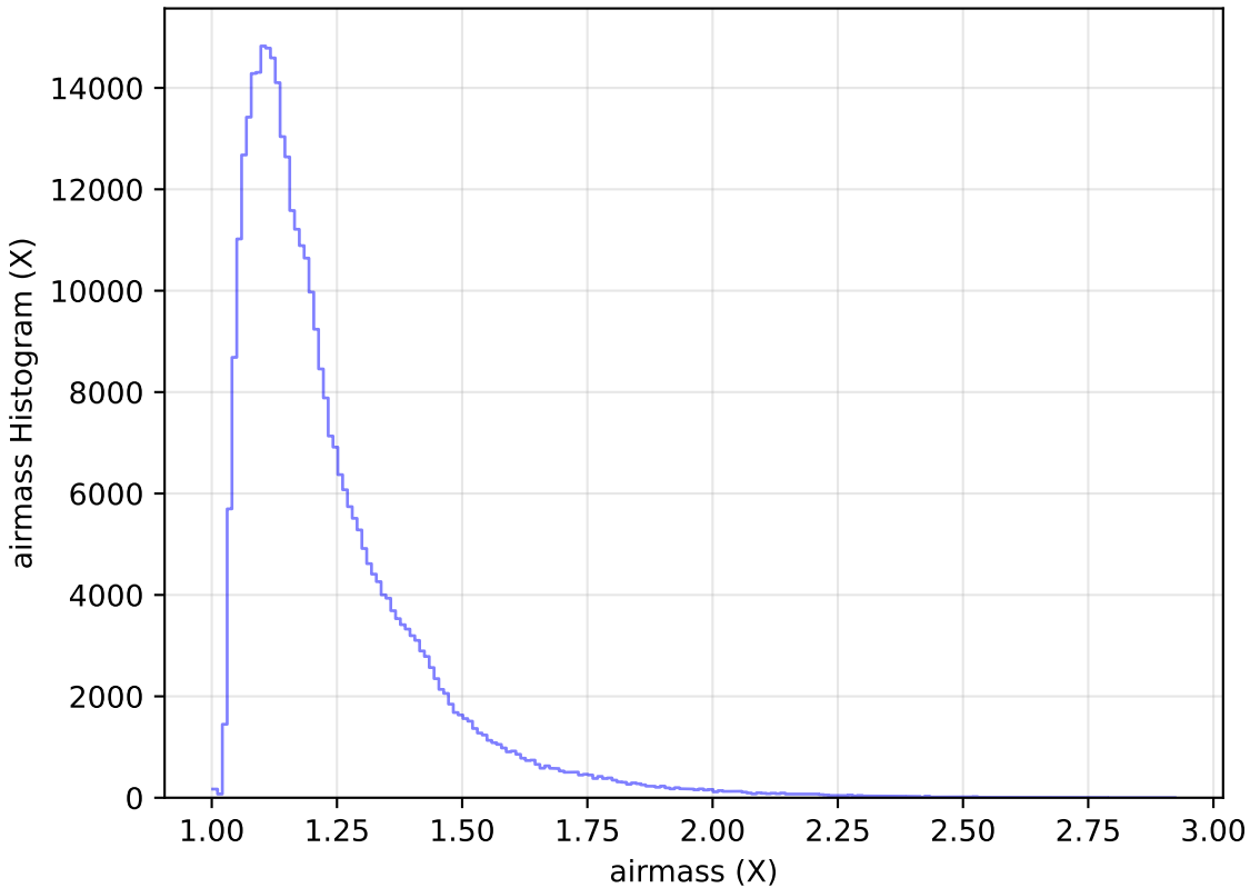
noroll_mjdp120_v3.4_10yrs WFD y band: airmass Histogram
