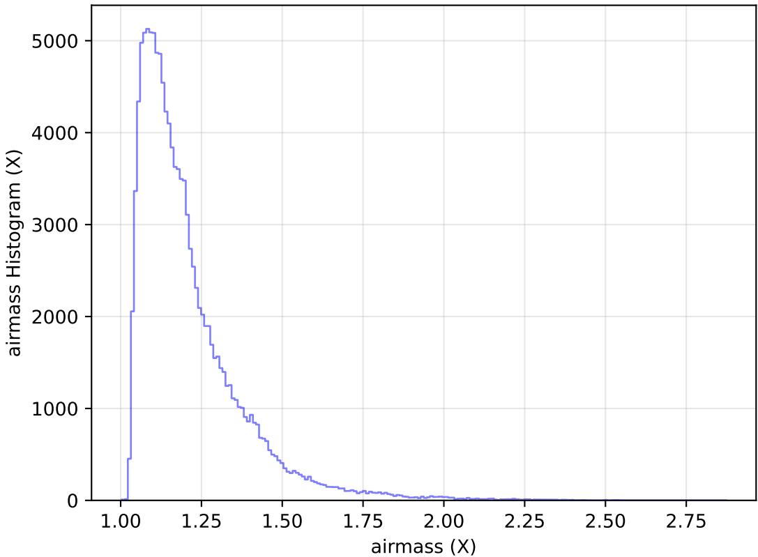
noroll_mjdp120_v3.4_10yrs WFD u band: airmass Histogram
