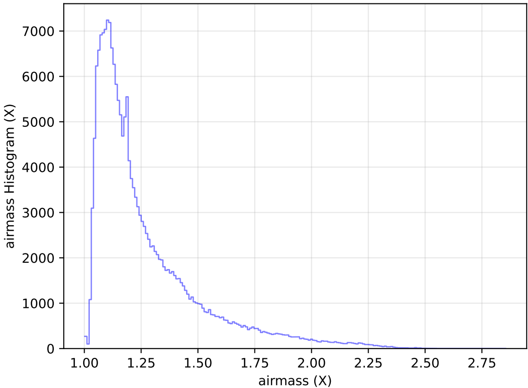
noroll_mjdp120_v3.4_10yrs WFD g band: airmass Histogram
