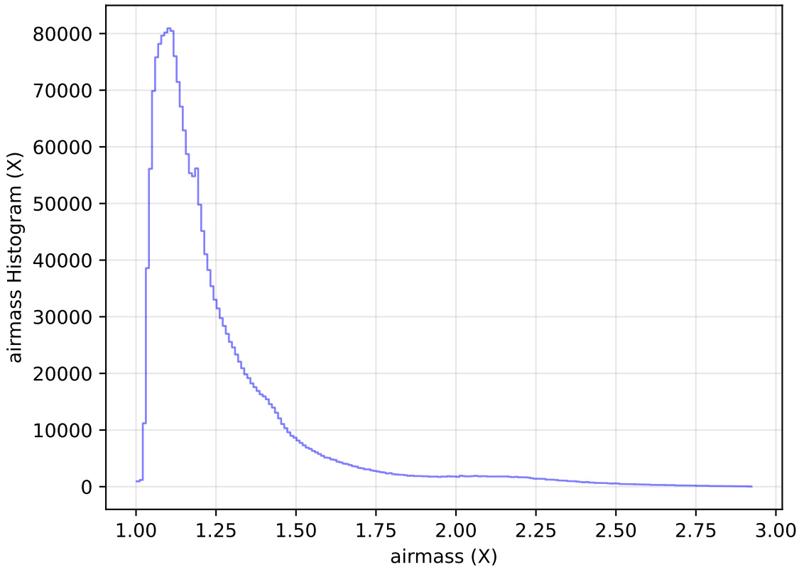
noroll_mjdp120_v3.4_10yrs WFD all bands: airmass Histogram
