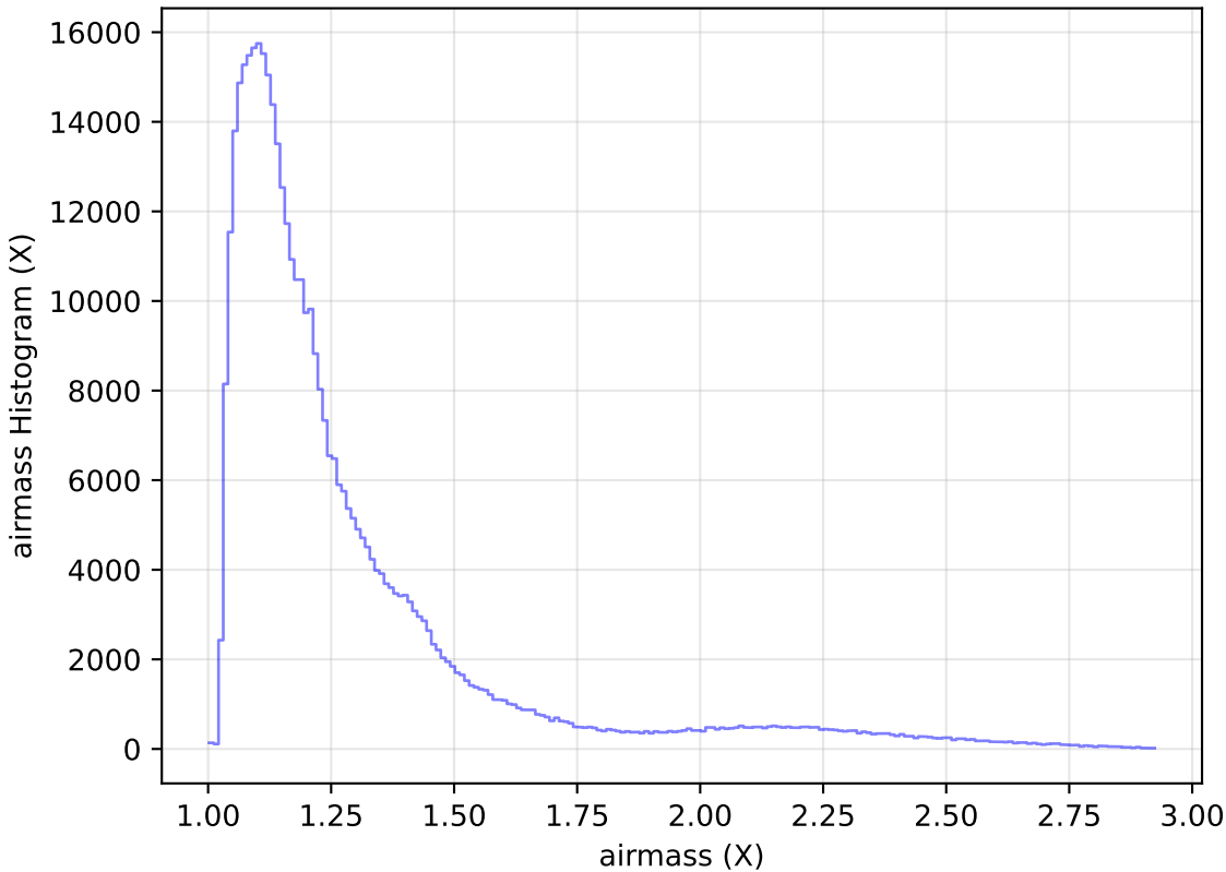
noroll_mjdp120_v3.4_10yrs All sky z band: airmass Histogram
