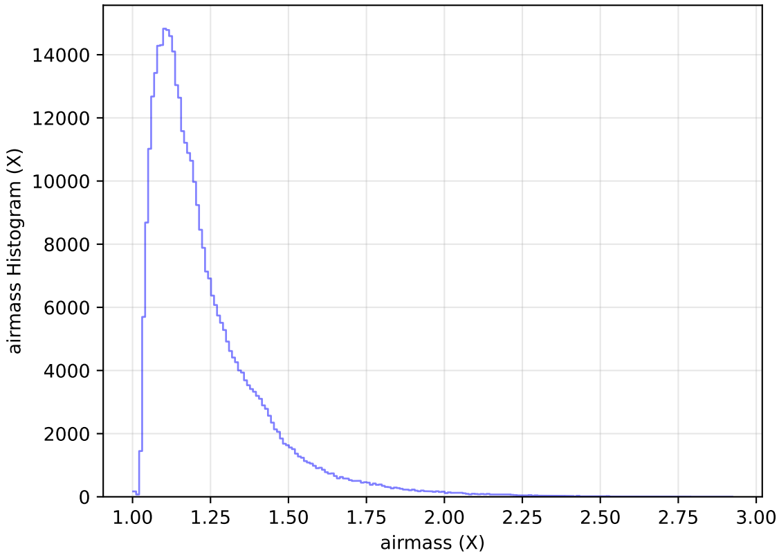
noroll_mjdp120_v3.4_10yrs All sky y band: airmass Histogram
