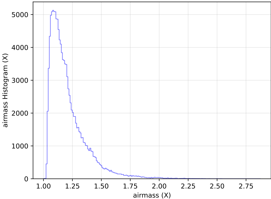
noroll_mjdp120_v3.4_10yrs All sky u band: airmass Histogram
