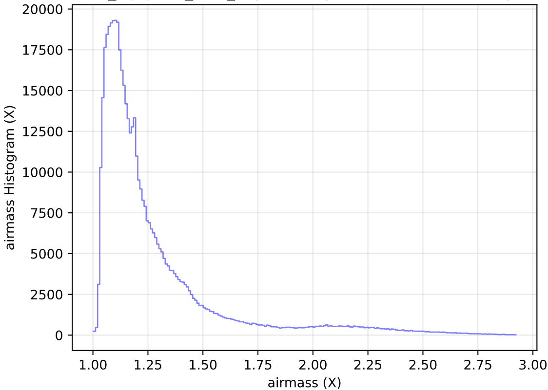
noroll_mjdp120_v3.4_10yrs All sky i band: airmass Histogram
