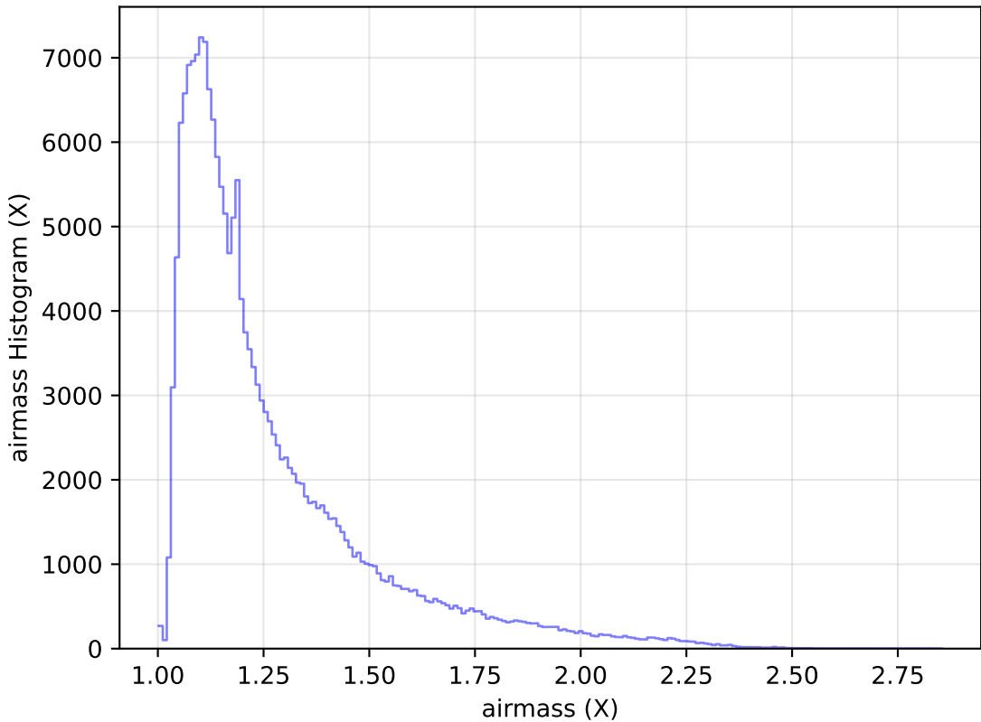
noroll_mjdp120_v3.4_10yrs All sky g band: airmass Histogram
