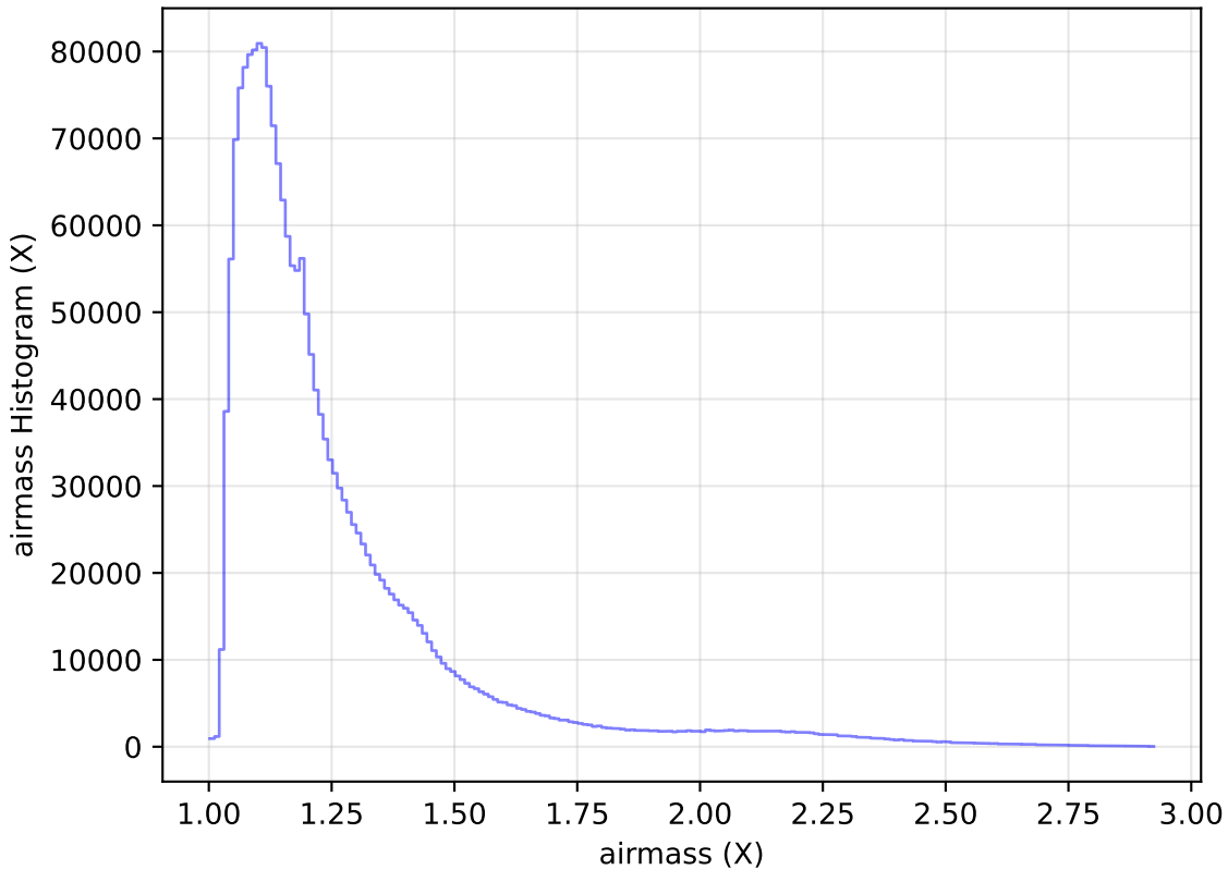
noroll_mjdp120_v3.4_10yrs All sky all bands: airmass Histogram
