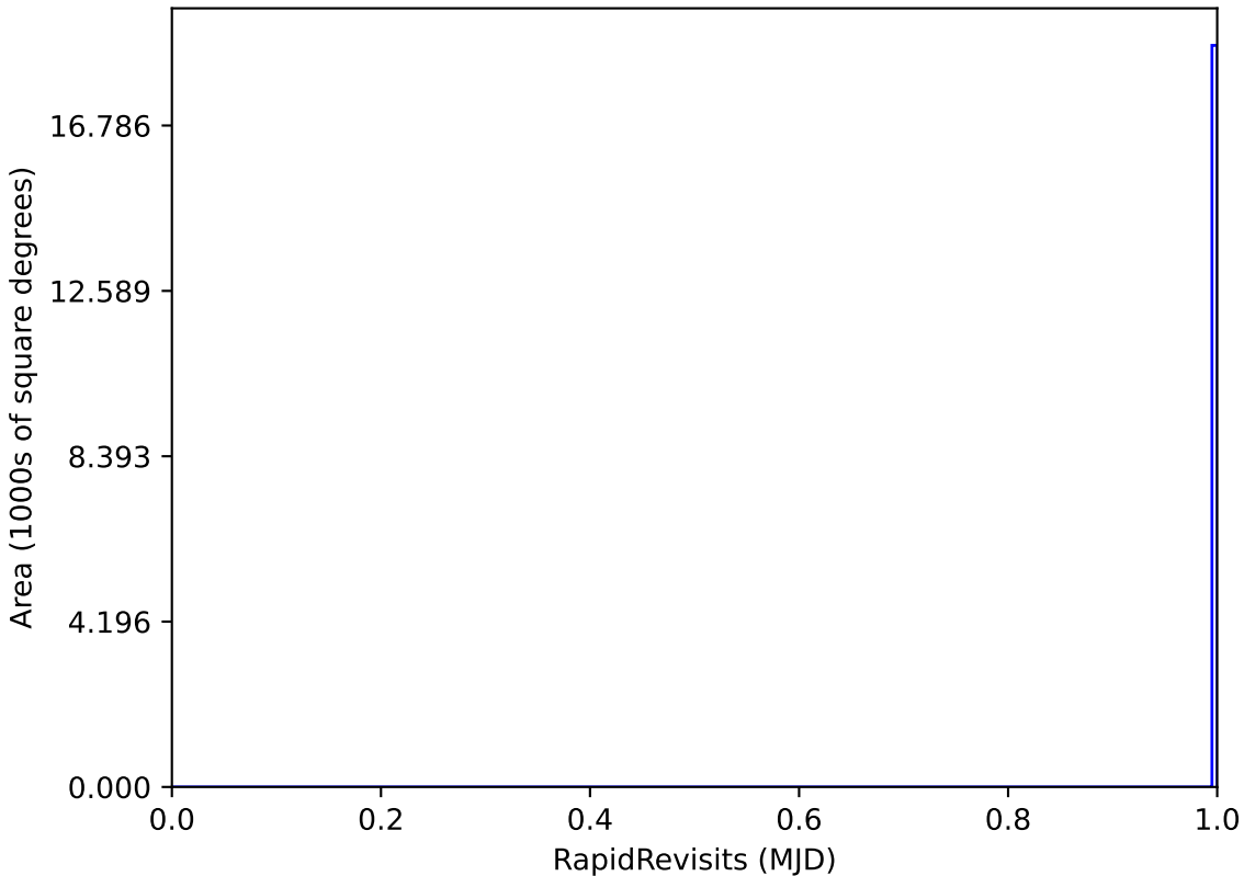
noroll_mjdp120_v3.4_10yrs WFD: RapidRevisits
