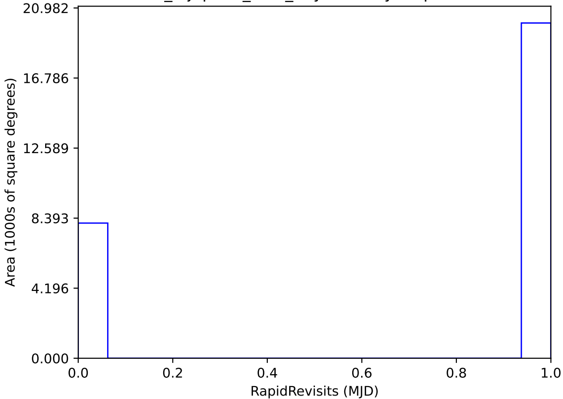
noroll_mjdp120_v3.4_10yrs All sky: RapidRevisits
