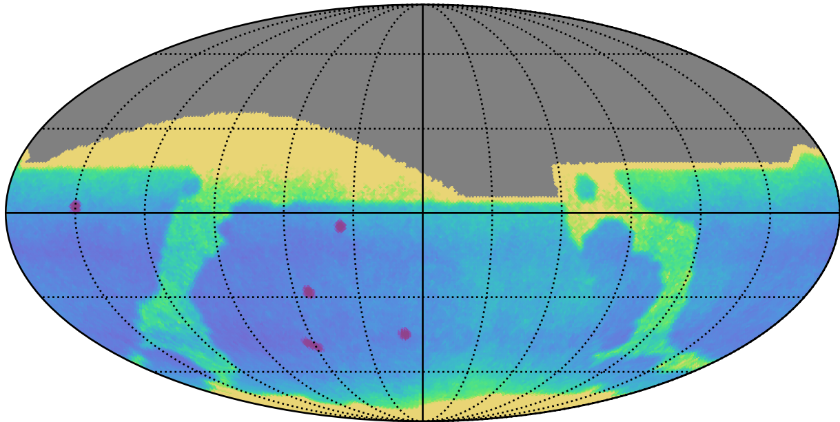
noroll_mjdp120_v3.4_10yrs All sky: Proper Motion Uncert @ 24.0
