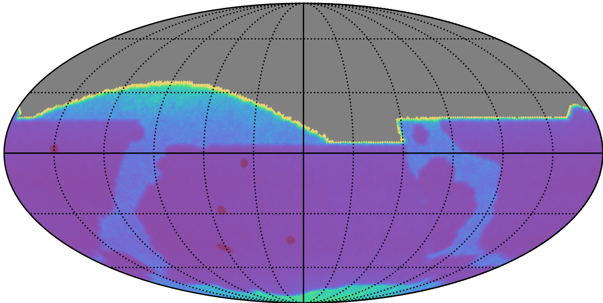
noroll_mjdp120_v3.4_10yrs All sky: Proper Motion Uncert @ 20.5
