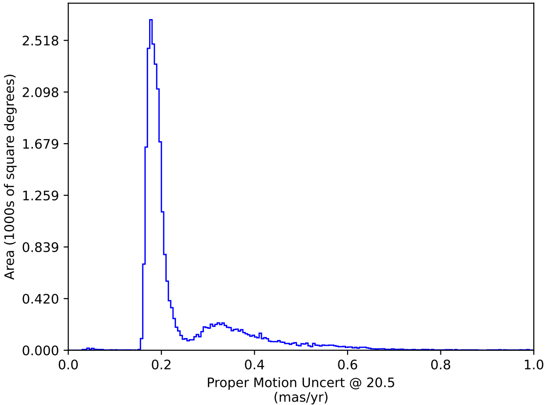
noroll_mjdp120_v3.4_10yrs All sky: Proper Motion Uncert @ 20.5
