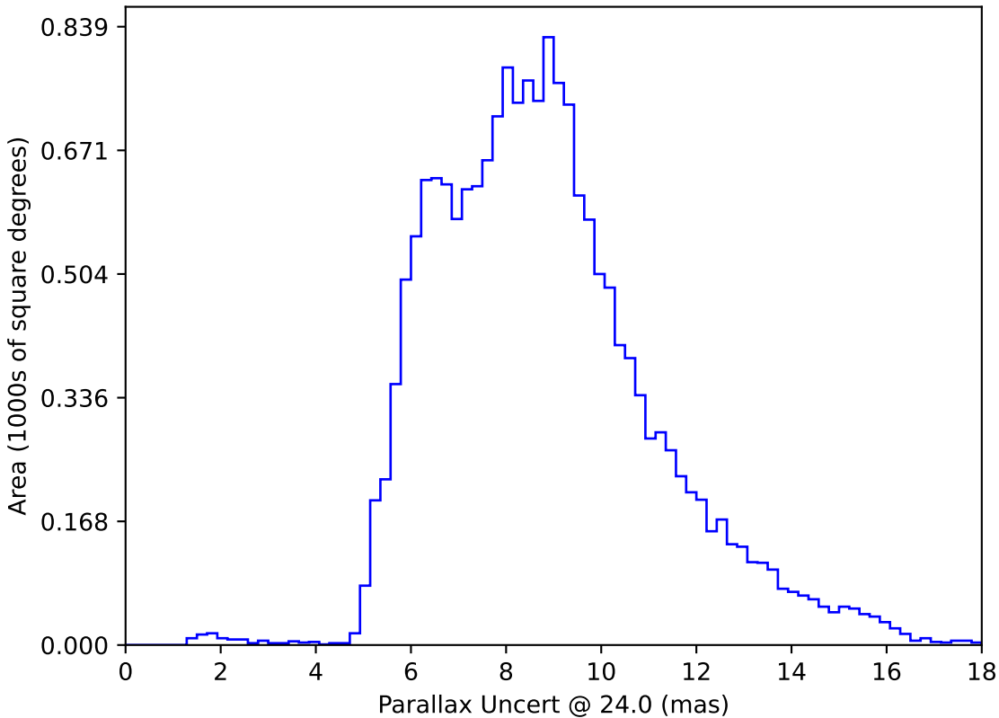
noroll_mjdp120_v3.4_10yrs WFD: Parallax Uncert @ 24.0
