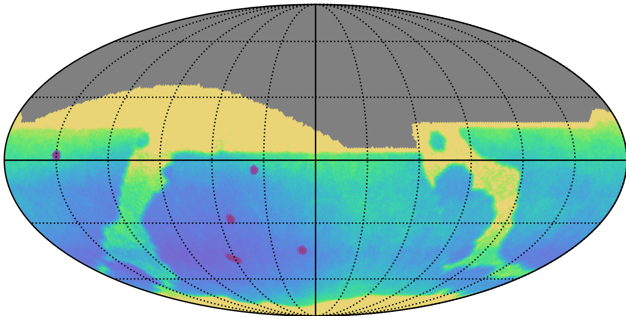
noroll_mjdp120_v3.4_10yrs All sky: Parallax Uncert @ 24.0
