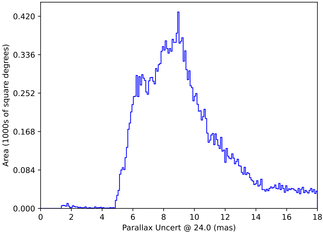
noroll_mjdp120_v3.4_10yrs All sky: Parallax Uncert @ 24.0
