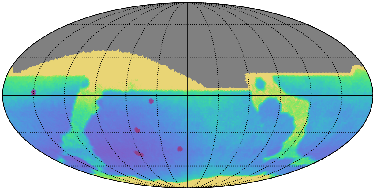
noroll_mjdp120_v3.4_10yrs All sky: Parallax Uncert @ 22.4
