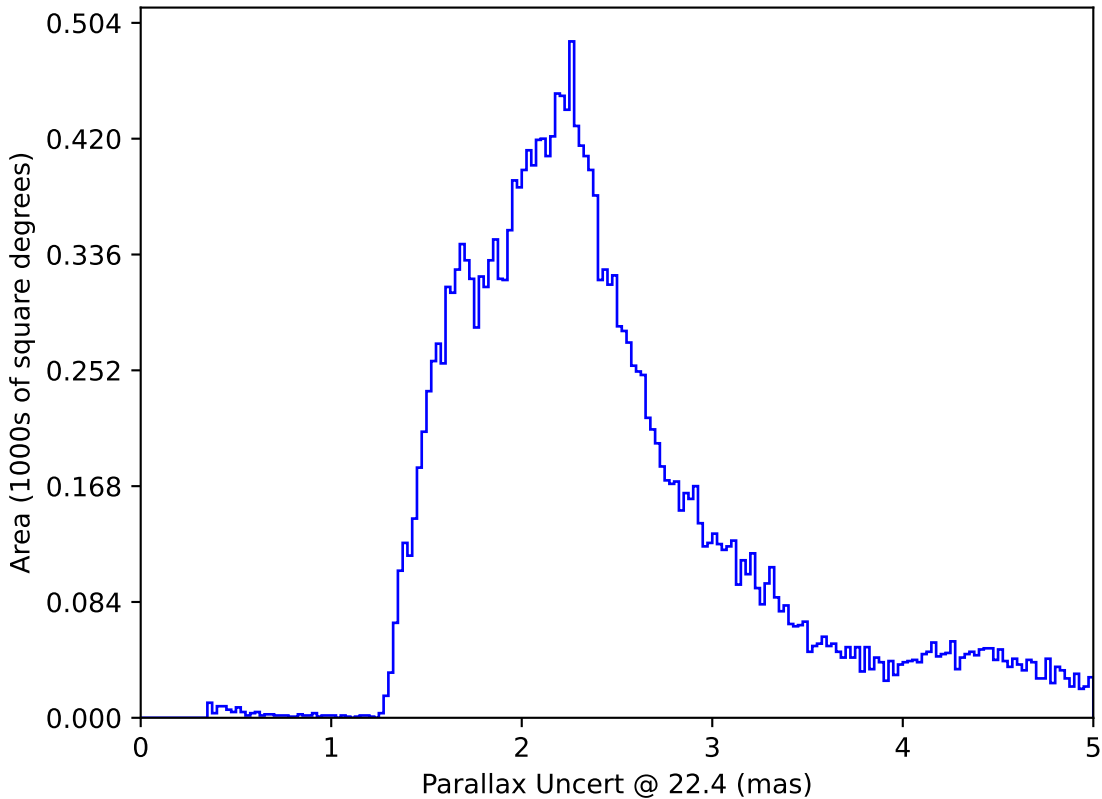
noroll_mjdp120_v3.4_10yrs All sky: Parallax Uncert @ 22.4
