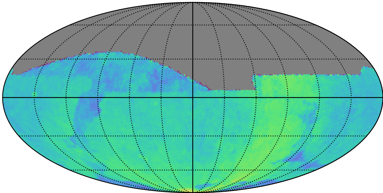
noroll_mjdp120_v3.4_10yrs All sky: Parallax Coverage @ 24.0
