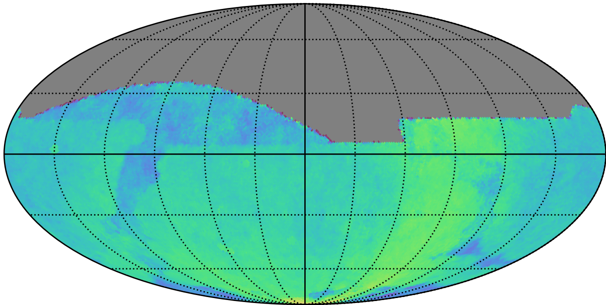
noroll_mjdp120_v3.4_10yrs All sky: Parallax Coverage @ 22.4
