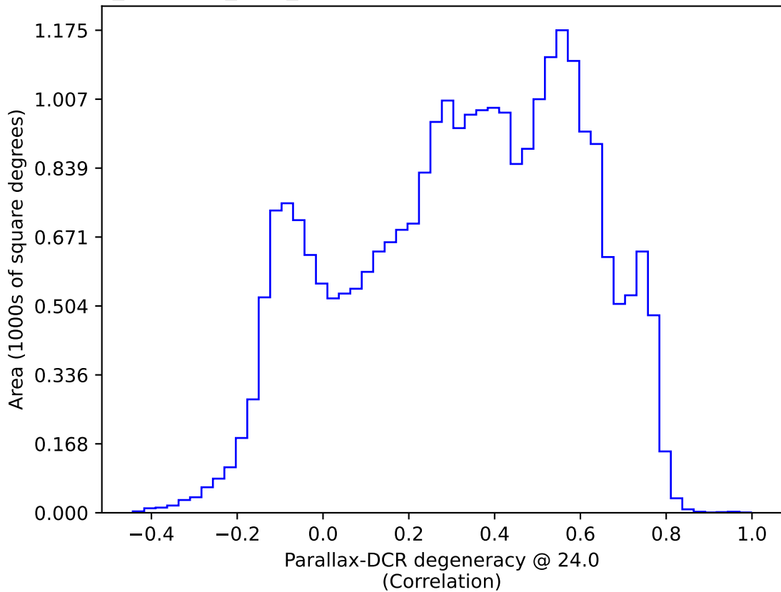
noroll_mjdp120_v3.4_10yrs All sky: Parallax-DCR degeneracy @ 24.0
