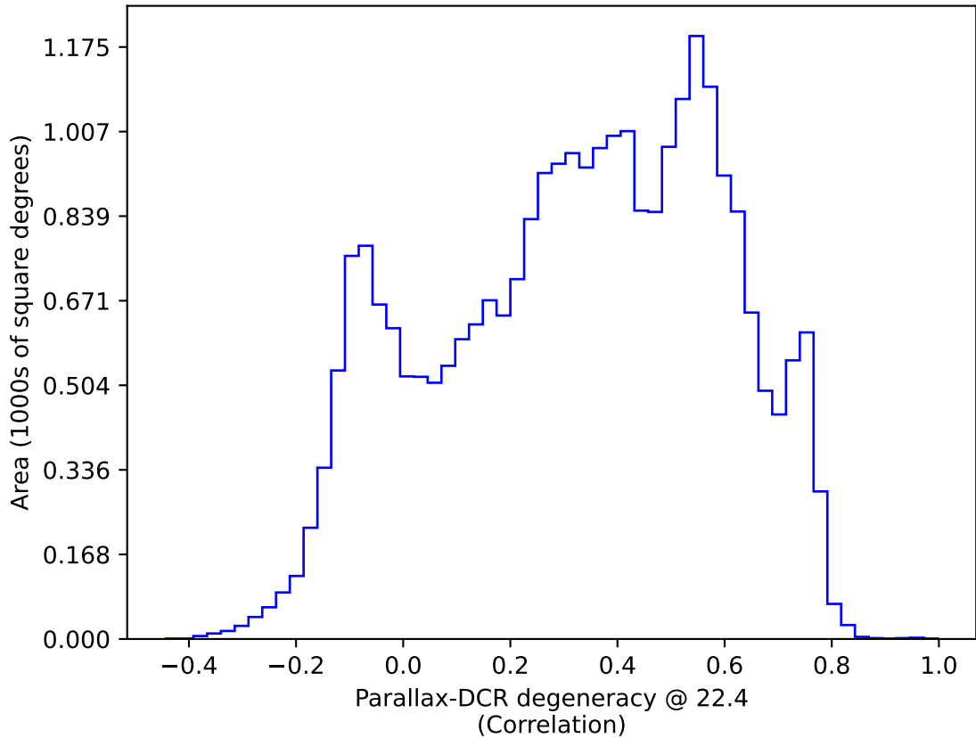
noroll_mjdp120_v3.4_10yrs All sky: Parallax-DCR degeneracy @ 22.4
