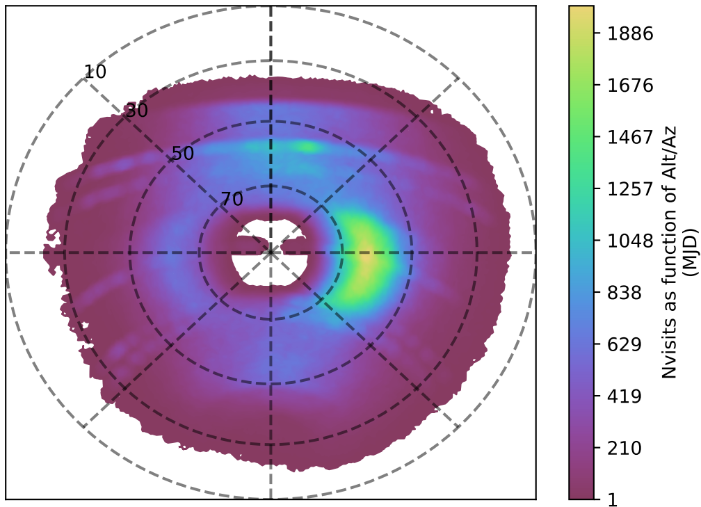
noroll_mjdp120_v3.4_10yrs y band: Nvisits as function of Alt/Az
