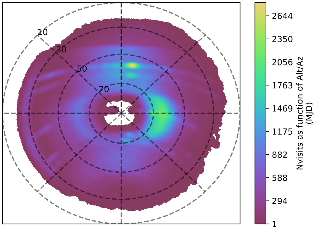
noroll_mjdp120_v3.4_10yrs r band: Nvisits as function of Alt/Az
