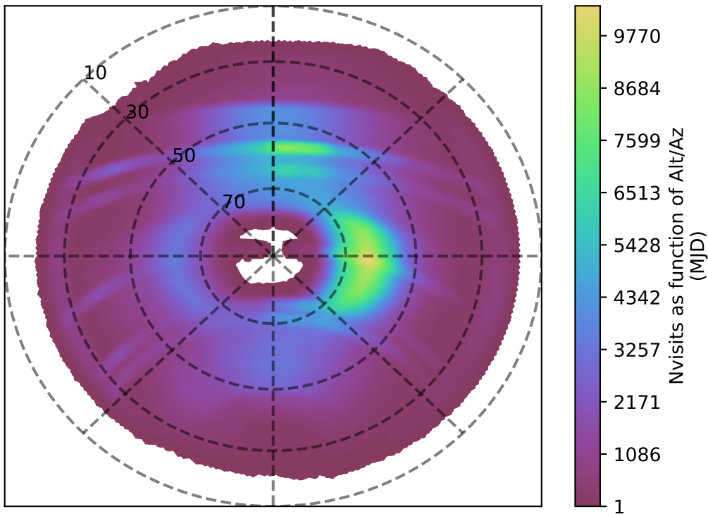
noroll_mjdp120_v3.4_10yrs all bands: Nvisits as function of Alt/Az
