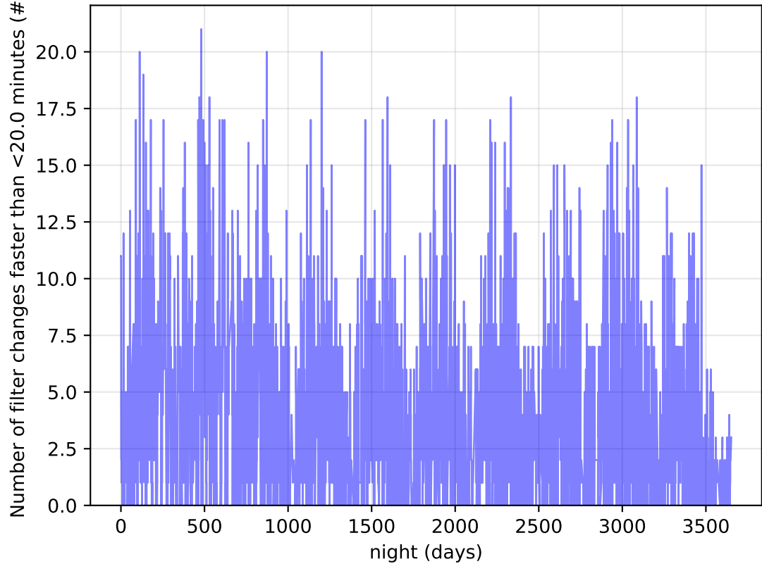
noroll_midp120_v3.4_10yrs Per Night: Number of filter changes faster than <20.0 minutes
