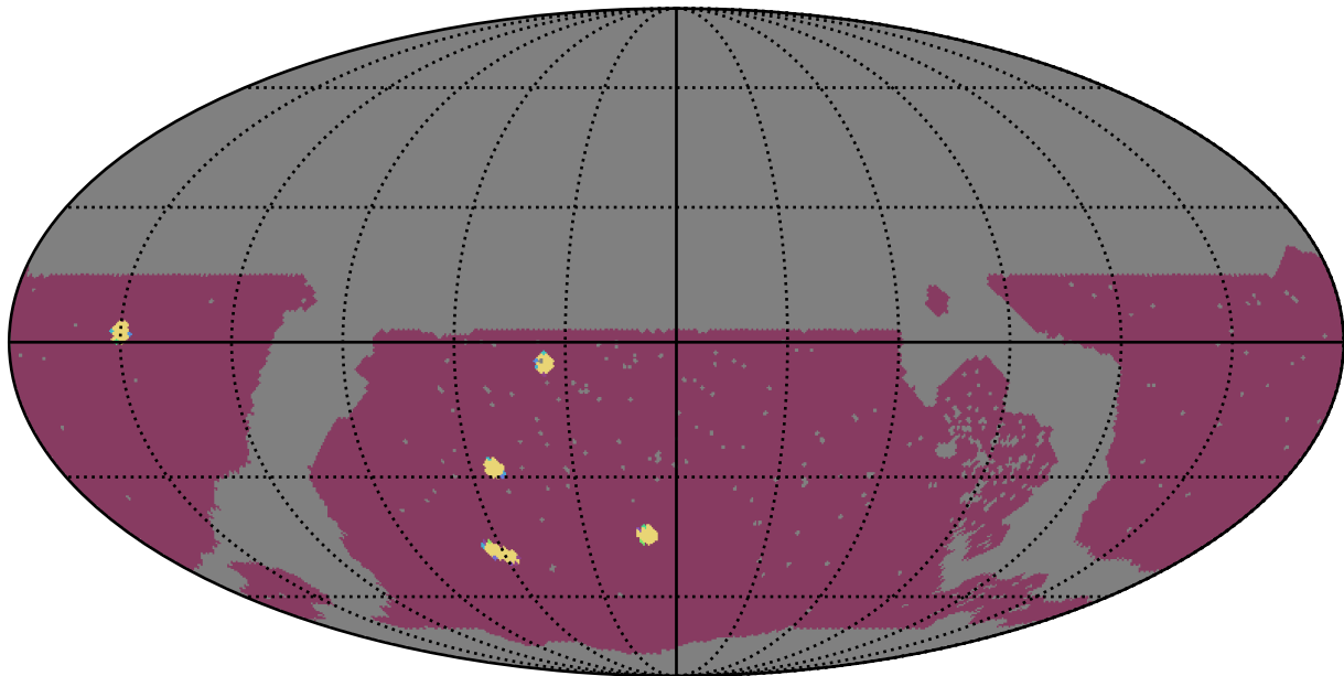
noroll_mjdp120_v3.4_10yrs WFD: NumberOfQuickRevisits
