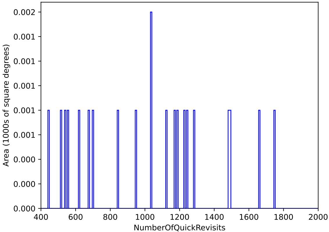
noroll_mjdp120_v3.4_10yrs WFD: NumberOfQuickRevisits
