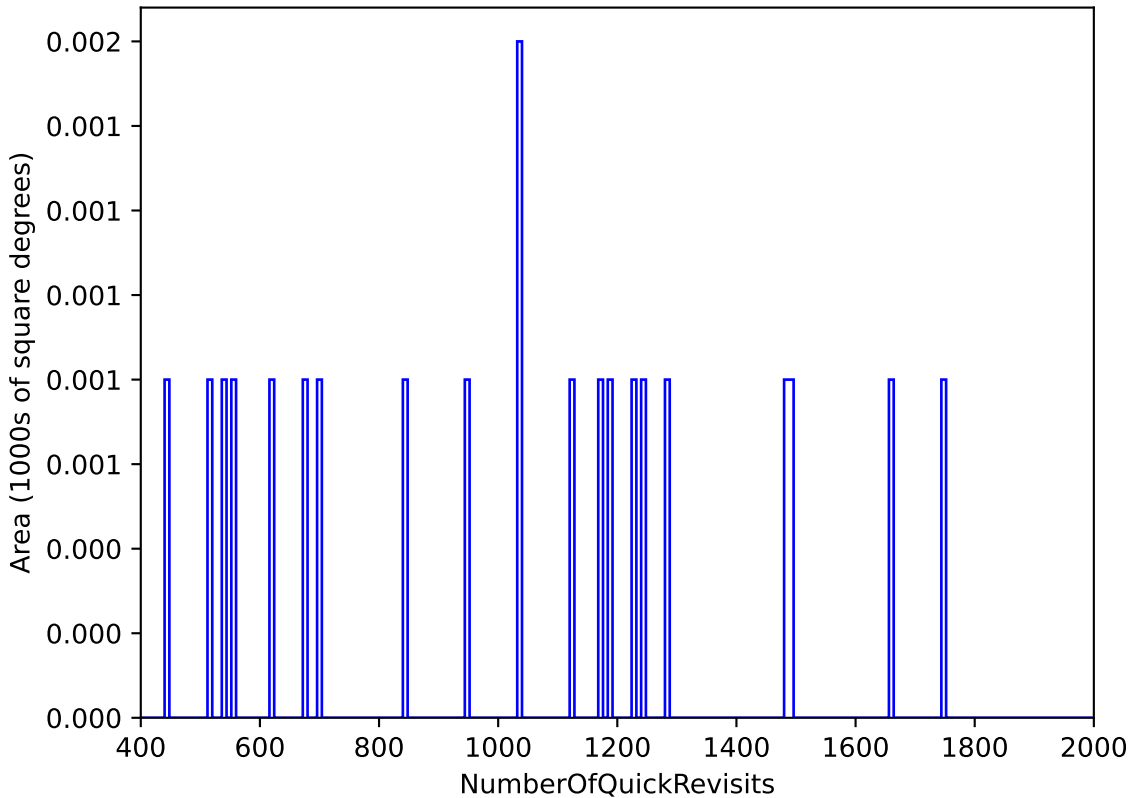
noroll_mjdp120_v3.4_10yrs All sky: NumberOfQuickRevisits
