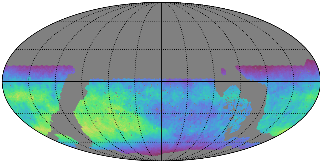
noroll_mjdp120_v3.4_10yrs WFD z band: Normalized Teff
