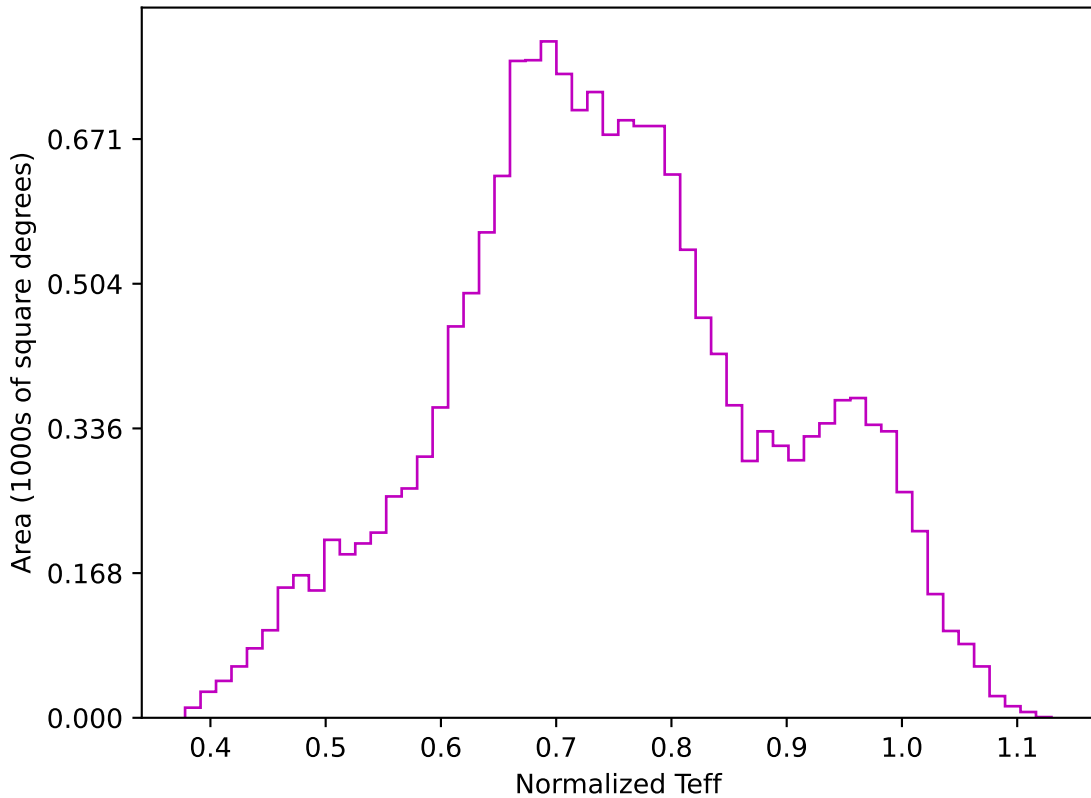
noroll_mjdp120_v3.4_10yrs WFD z band: Normalized Teff
