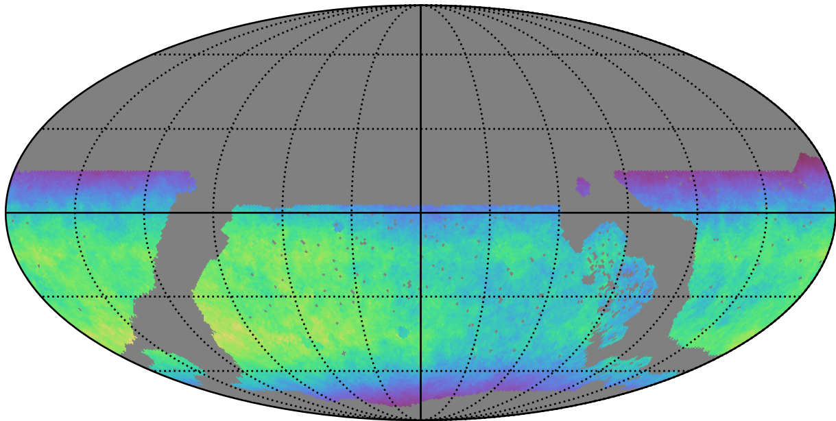
noroll_mjdp120_v3.4_10yrs WFD y band: Normalized Teff
