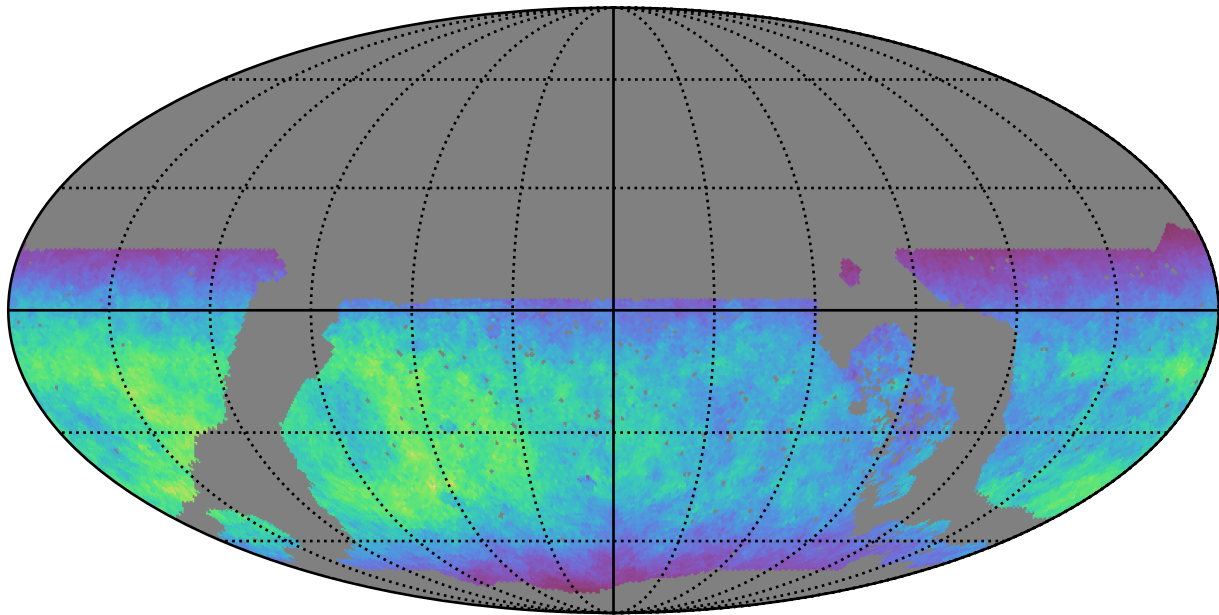
noroll_mjdp120_v3.4_10yrs WFD u band: Normalized Teff
