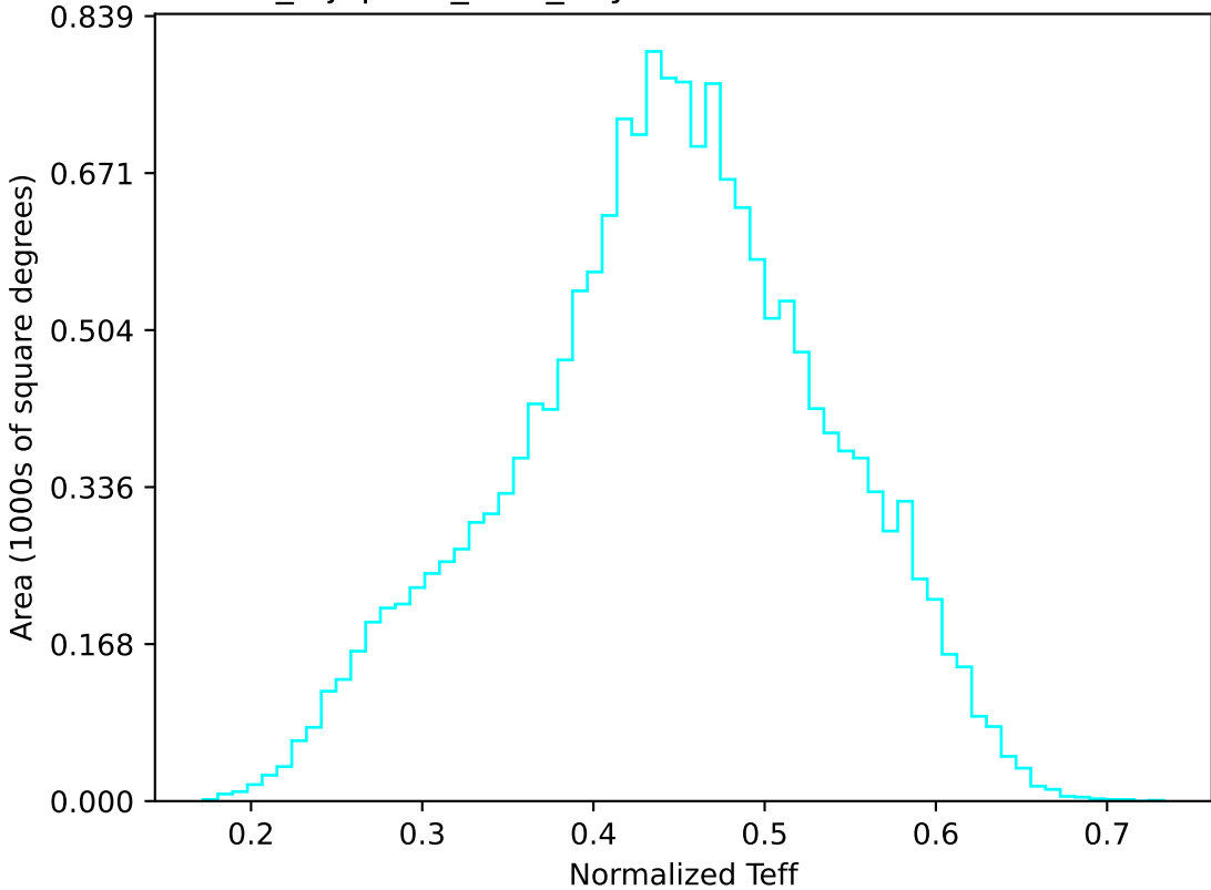
noroll_mjdp120_v3.4_10yrs WFD u band: Normalized Teff
