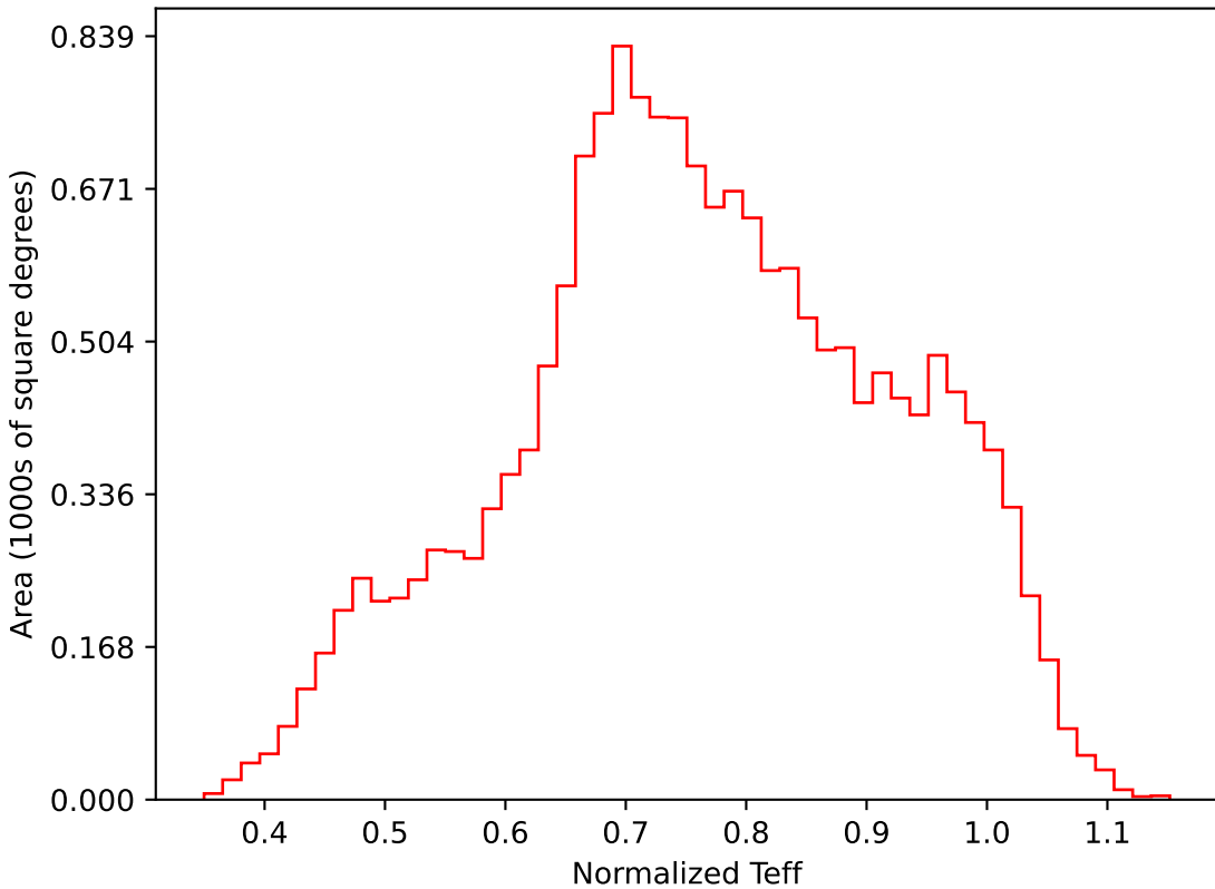
noroll_mjdp120_v3.4_10yrs WFD i band: Normalized Teff
