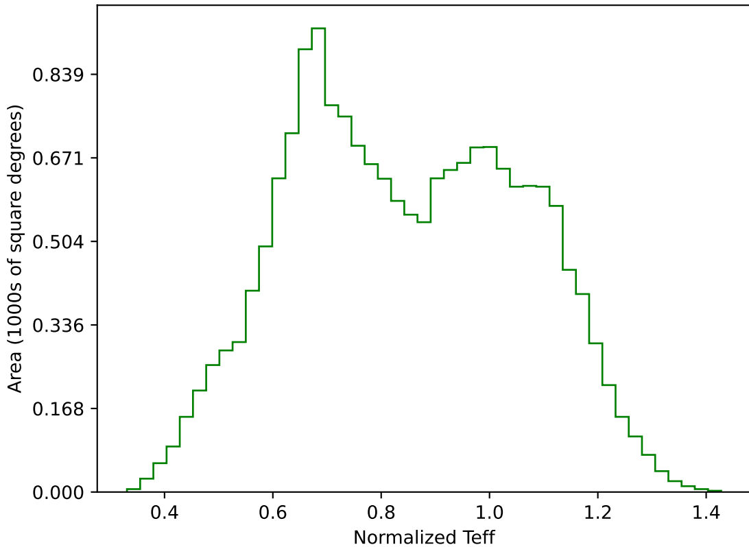
noroll_mjdp120_v3.4_10yrs WFD g band: Normalized Teff
