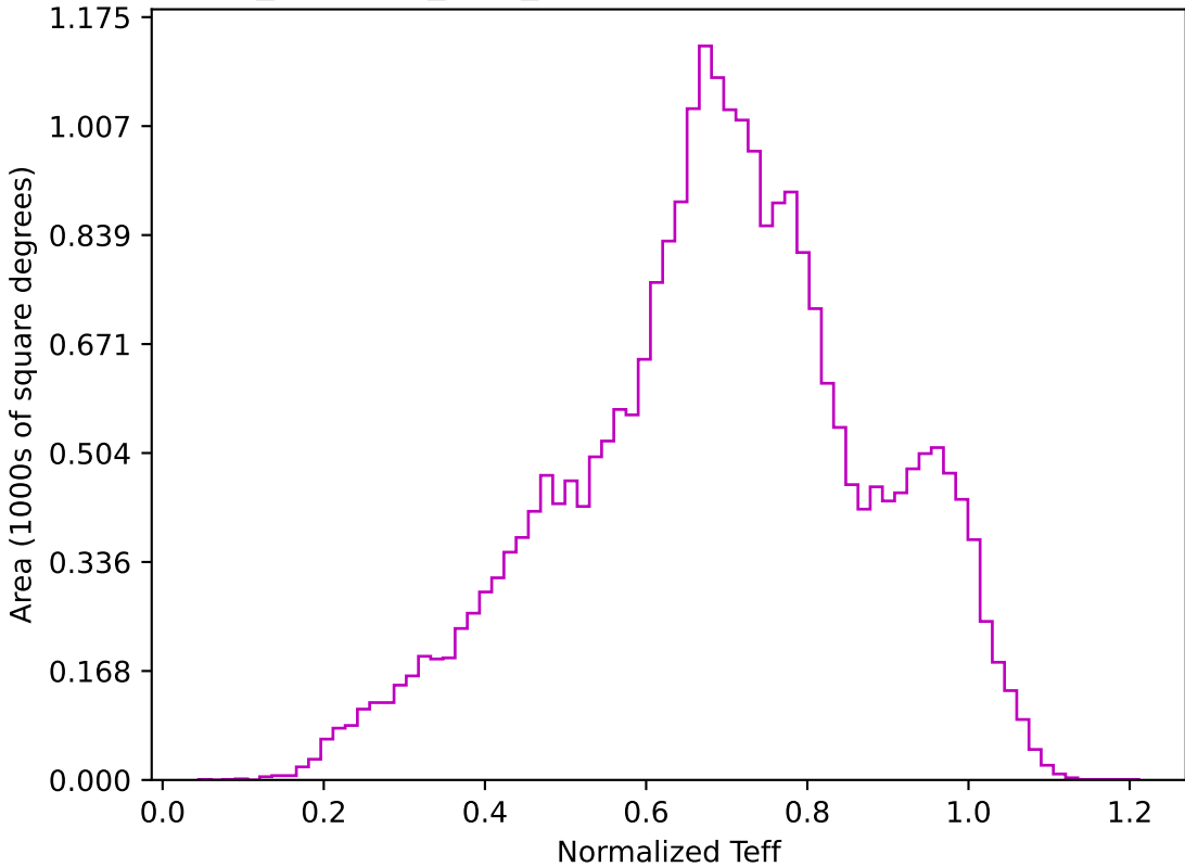
noroll_mjdp120_v3.4_10yrs All sky z band: Normalized Teff
