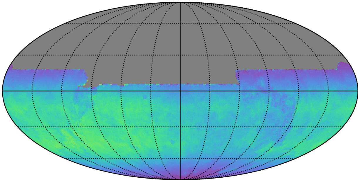
noroll_mjdp120_v3.4_10yrs All sky y band: Normalized Teff
