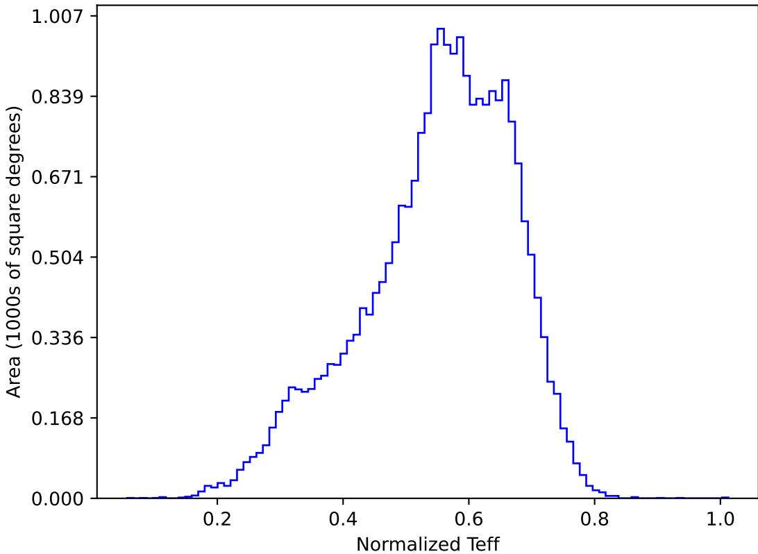
noroll_mjdp120_v3.4_10yrs All sky y band: Normalized Teff
