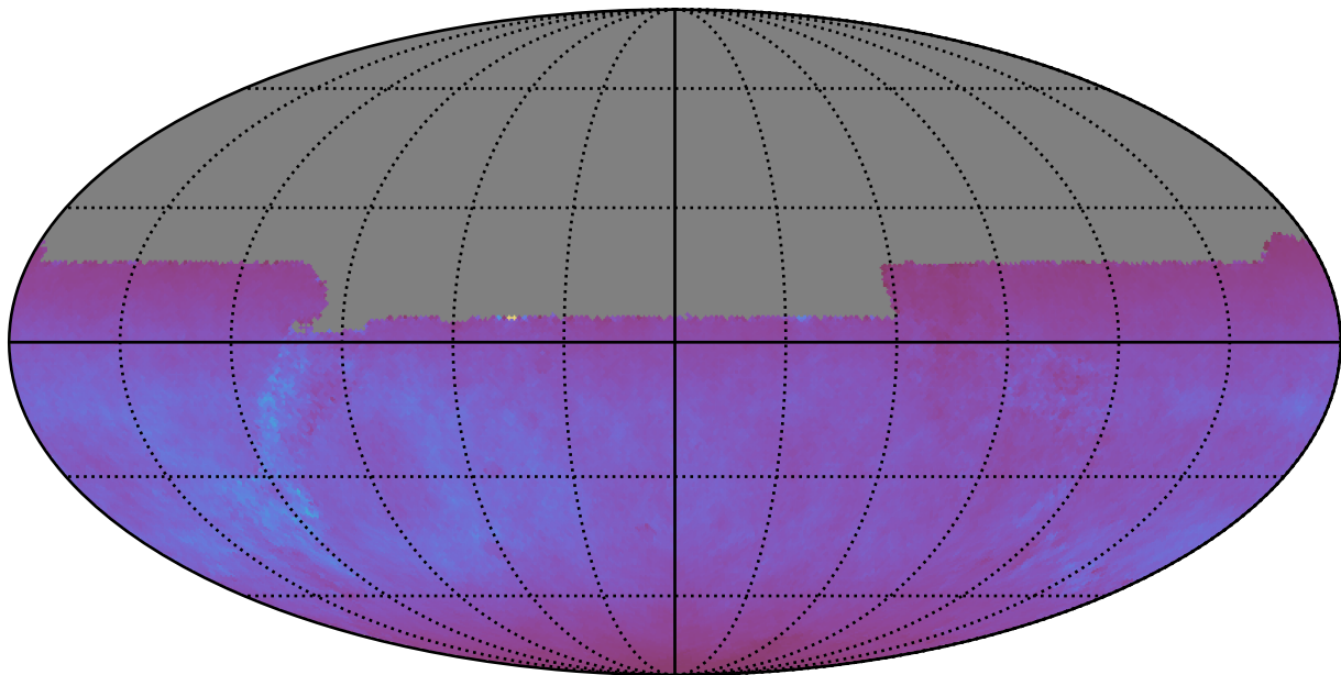
noroll_mjdp120_v3.4_10yrs All sky u band: Normalized Teff
