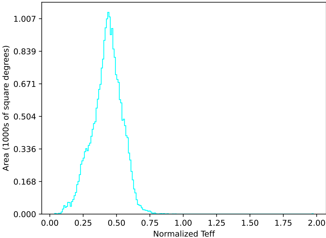
noroll_mjdp120_v3.4_10yrs All sky u band: Normalized Teff
