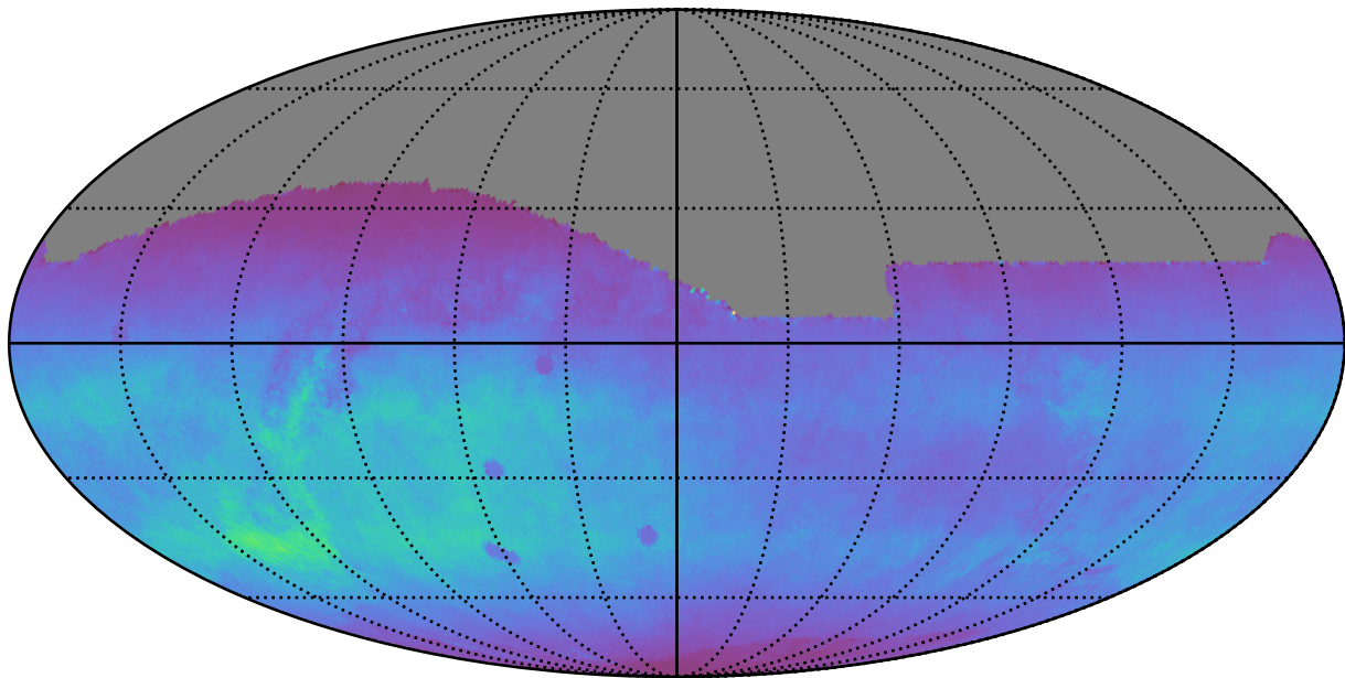
noroll_mjdp120_v3.4_10yrs All sky r band: Normalized Teff
