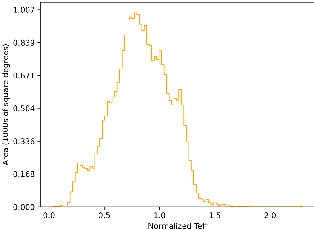
noroll_mjdp120_v3.4_10yrs All sky r band: Normalized Teff
