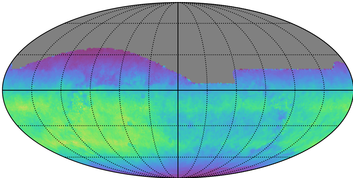
noroll_mjdp120_v3.4_10yrs All sky i band: Normalized Teff
