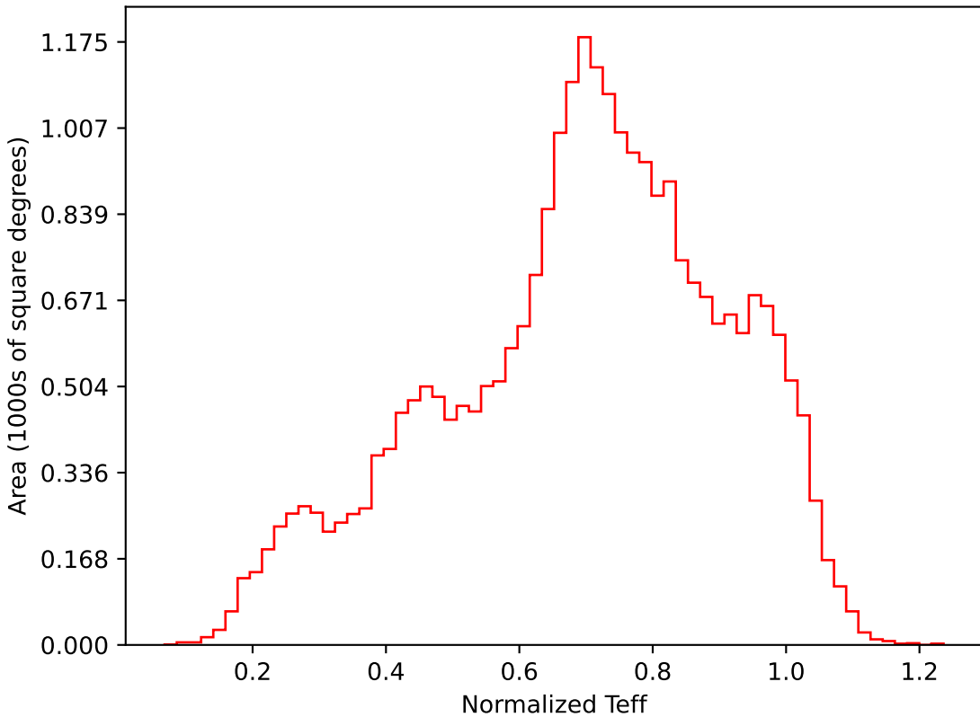
noroll_mjdp120_v3.4_10yrs All sky i band: Normalized Teff
