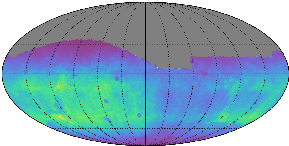
noroll_mjdp120_v3.4_10yrs All sky g band: Normalized Teff
