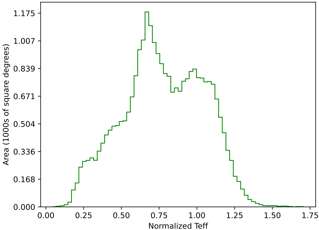
noroll_mjdp120_v3.4_10yrs All sky g band: Normalized Teff
