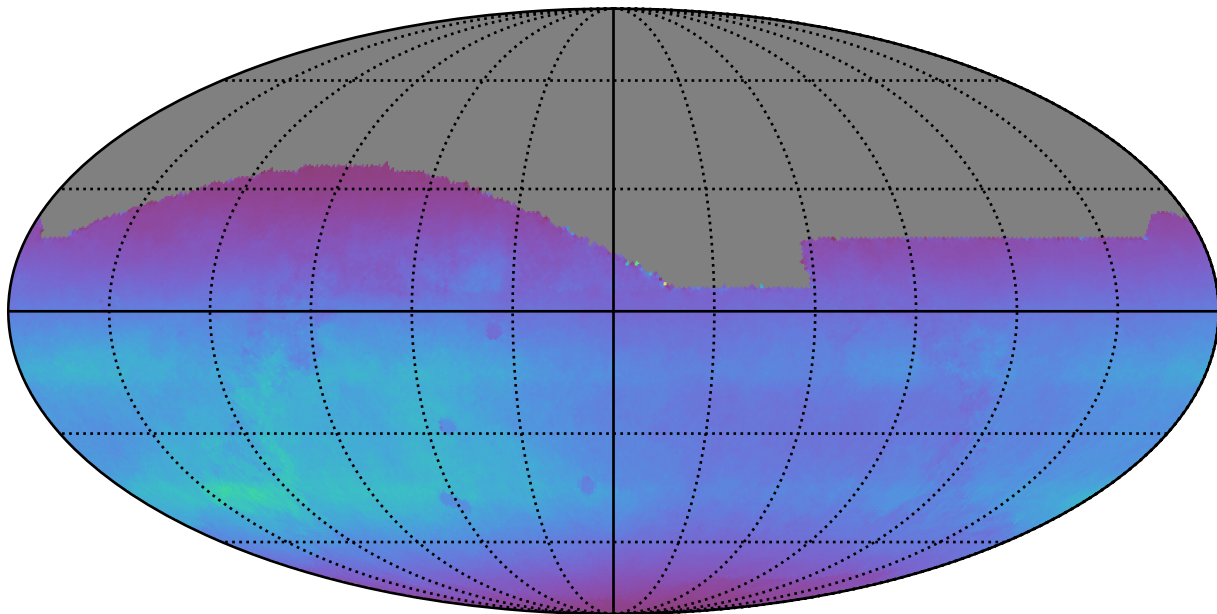
noroll_mjdp120_v3.4_10yrs All sky all bands: Normalized Teff
